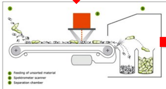
Triboelectric/NIR/metal sorting
